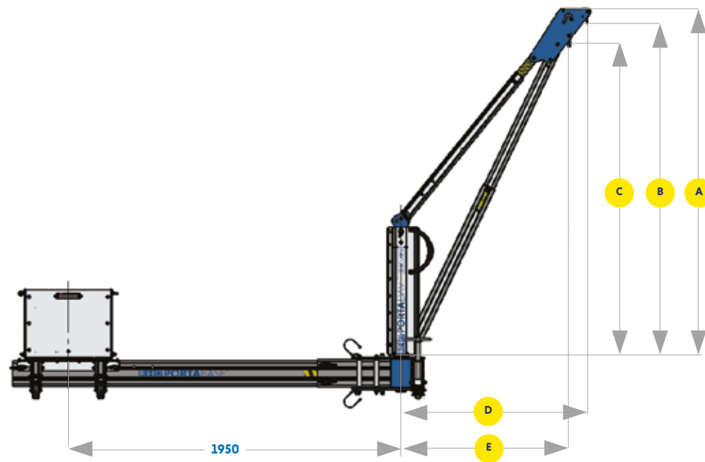
DIMENSIONS (MM)
